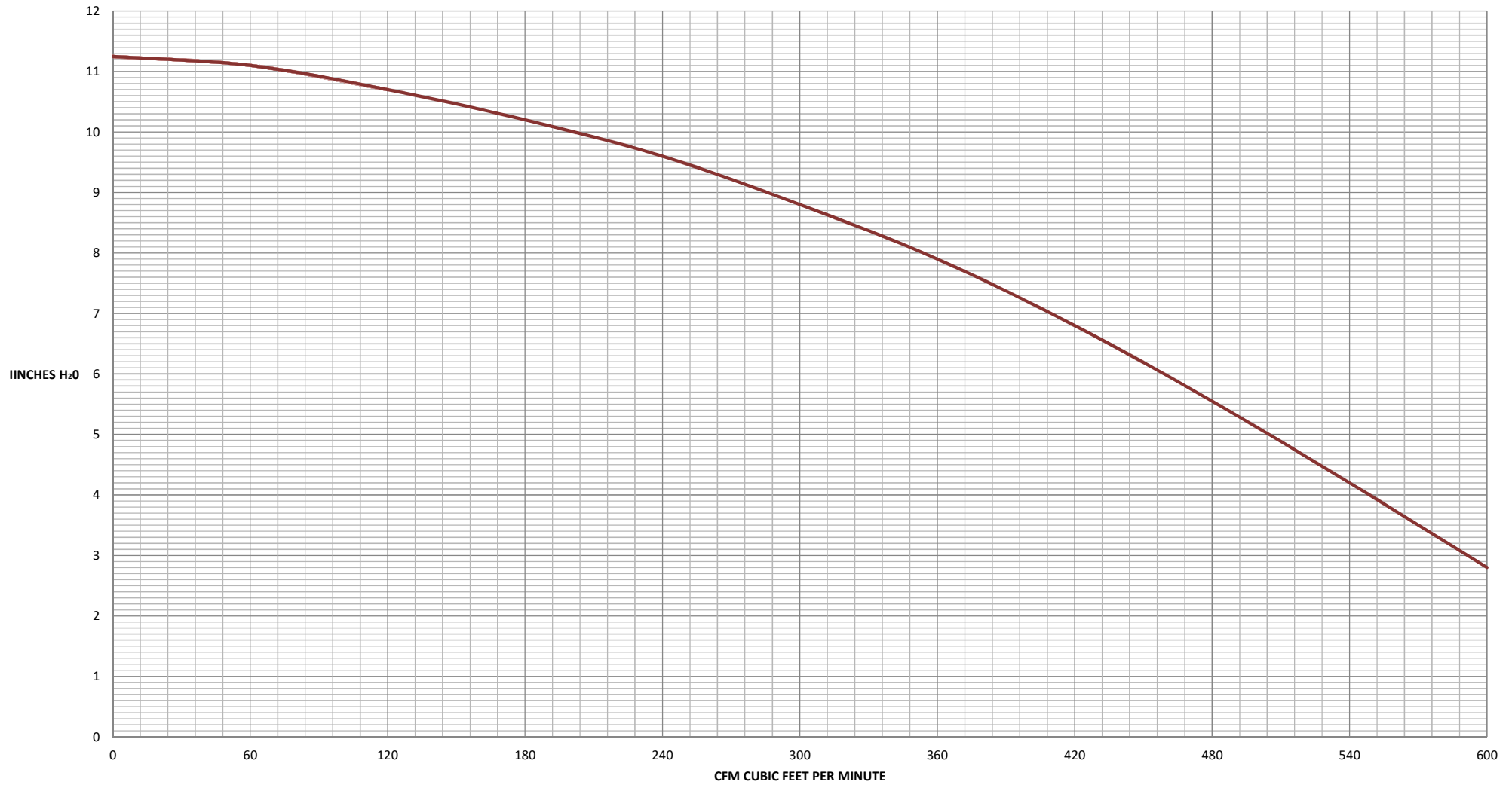
PERFORMANCE CURVE MODEL CD-600 EX / TV-600 @ 60Hz
